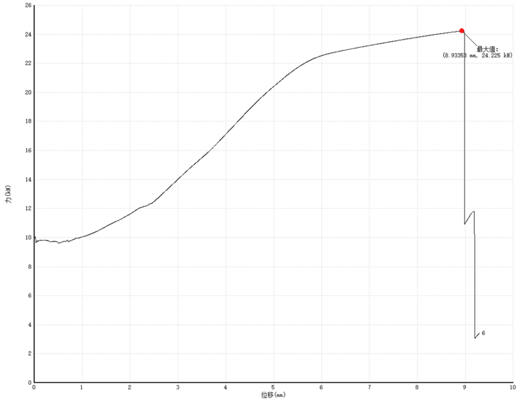
Force-displacement curve
